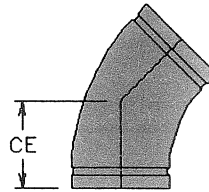
45 ELBOWS LR
