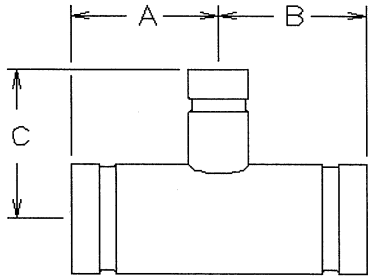
GROOVED REDUCING TEE
